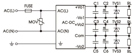
Fig. 2 LHE20-20Cxx series, typical circuit diagram
